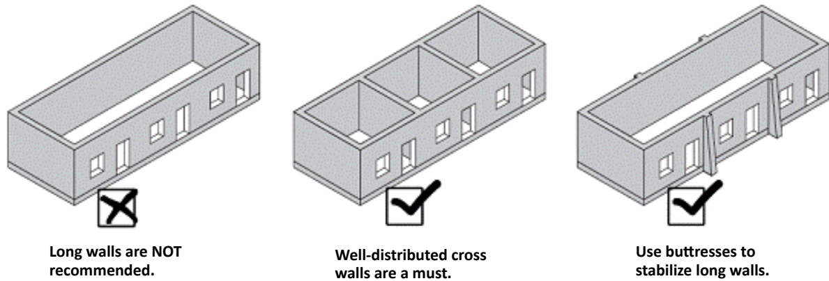
Figure 3.24 Recommendations related to the wall length (source: Bothara et al. 2002)
