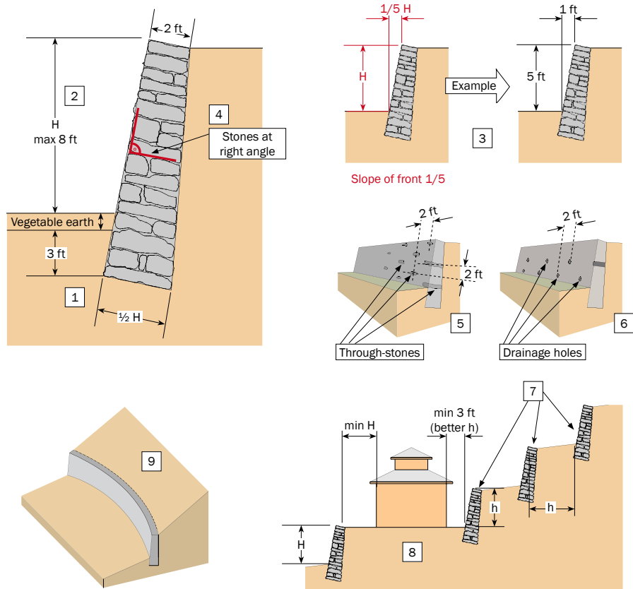
Figure 3.2 Special provisions for building construction on a steep slope (source: Schacher 2009)
