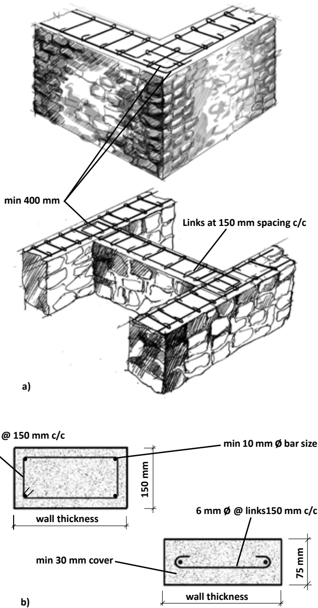
Figures 3.16 RC seismic bands: a) reinforcement layout, and b) cross-section of RC bands with 2 and 4 bars (adapted from: GOM 1998)
