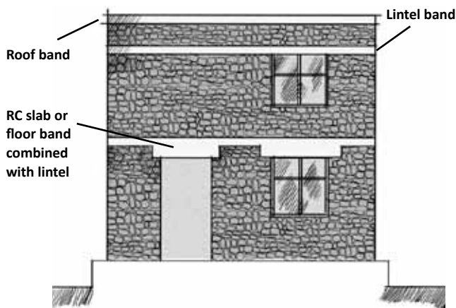
Figure 3.12 Merging RC floor and lintel bands
