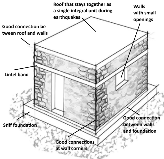
Figure 3.6 Key requirements for ensuring box action in a stone masonry building (adapted from: Murty 2005)
