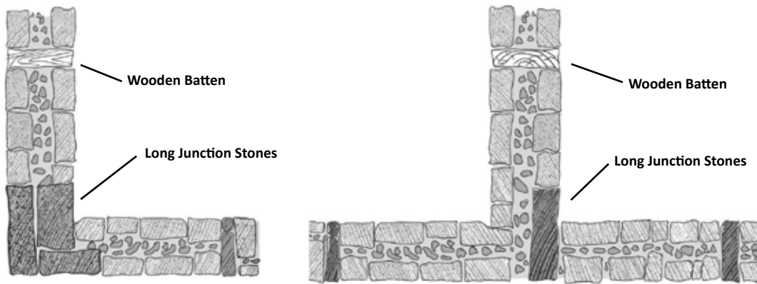
Figure 3.30 Placement of long stones at wall intersections (adapted from: Bothara et al. 2002)
