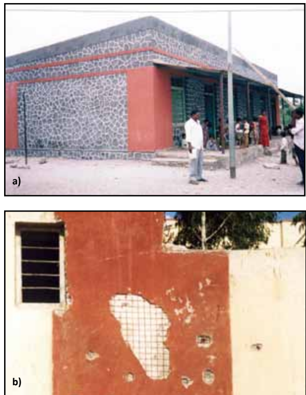
Figure 4.11 Strengthening of intersecting walls: a) retrofitted school building in India, and b) an unsuccessful retrofit application (photos: S. Brzev)
