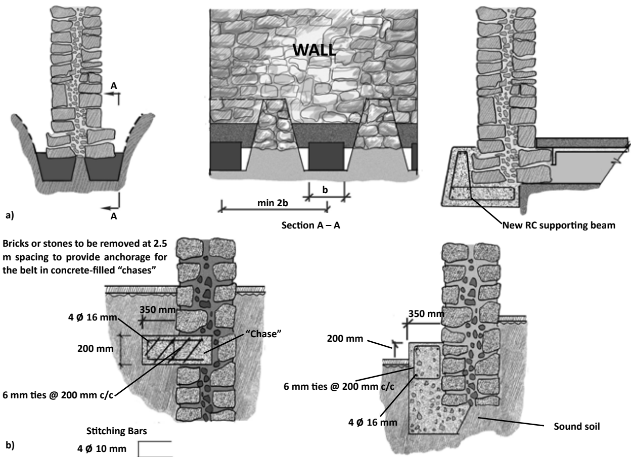
Figure 4.29 Strengthening existing foundations: a) underpinning the foundation, and b) external RC belt (adapted from: GOM 1998 and UNIDO 1983)
