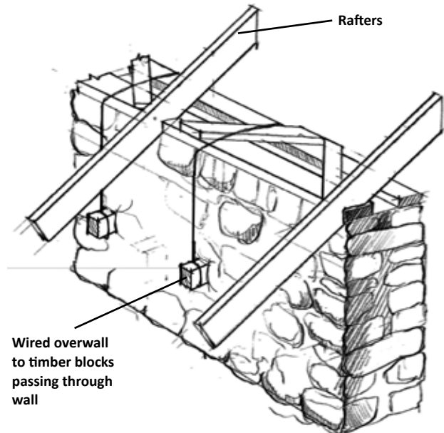
Figure 3.22 Timber band as a horizontal truss with cross members placed at a 45° angle to ensure roof anchorage
