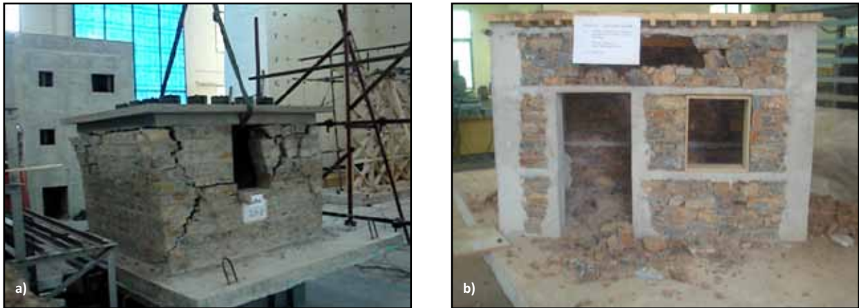
Figure 2.12 Damaged models at the end of the test: a) failure of model SM1, and b) model SM3 at the end of the experiment (source: Ali et al. 2010)
