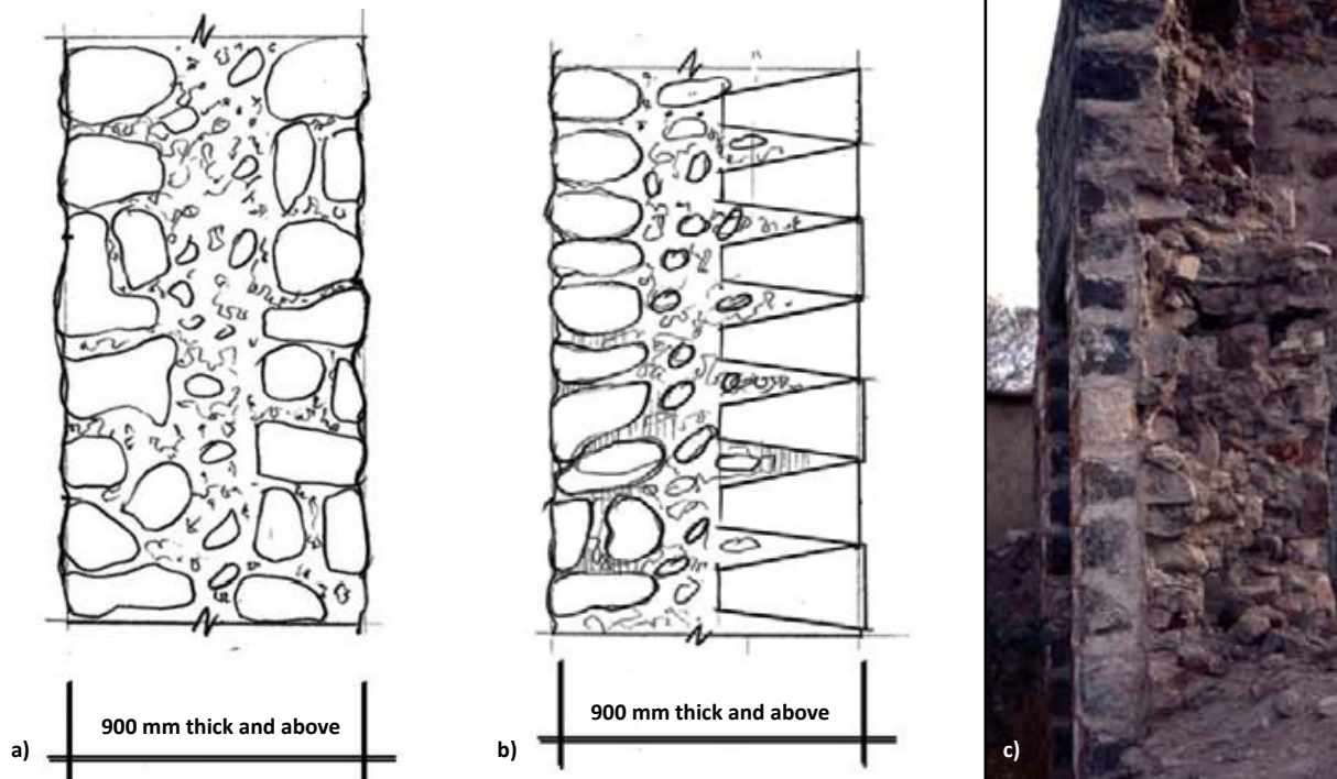
Figure 1.28 Stone masonry walls in Maharashtra, India: a) an uncoursed random rubble stone masonry wall (source: CBRI 1994); b) a semi-dressed stone wall with an exterior wythe built using wedge-shaped dressed stone (Source: CBRI, 1994), and c) (right) an example of a semi-dressed stone wall (photo: S. Brzev)
