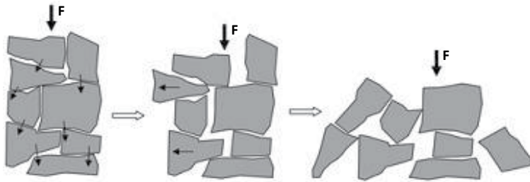
Figure 2.35b Detail of wall failure caused by irregular stones (source: Bothara and Hiçyılmaz 2008)
