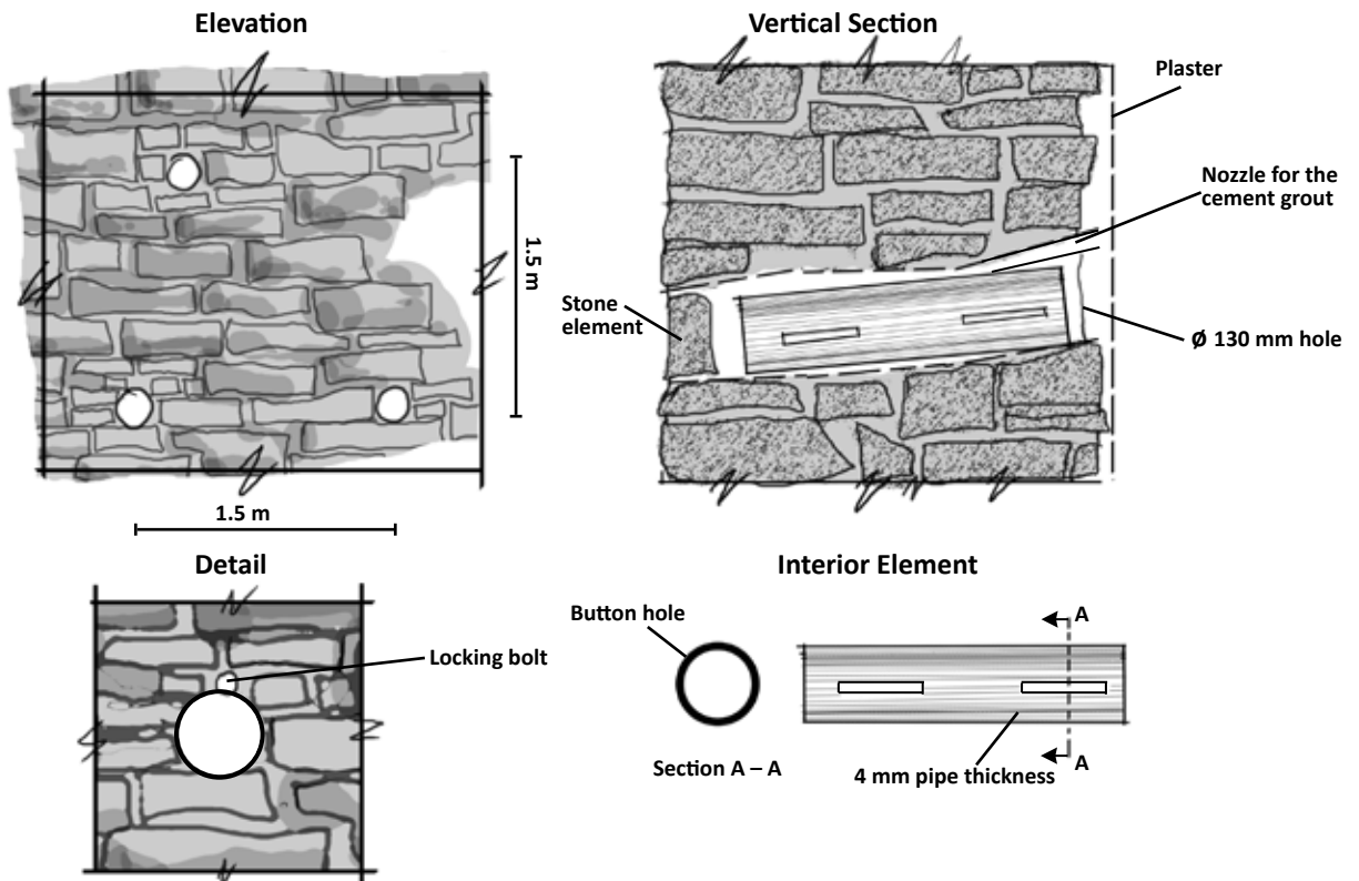
Figure 4.21 Installation of though-wall anchors in stone masonry walls after the 2002 Molise, Italy, earthquake (source: Maffei et al. 2006)
