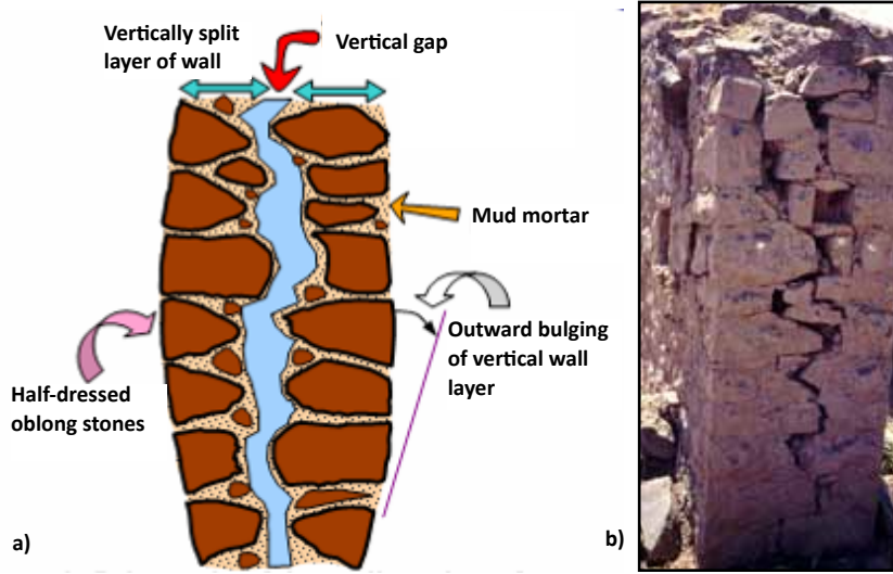
Figure 2.20 Delamination of stone masonry walls: a) delamination in progress (source: Murty 2005), and b) (right) delamination of wall wythes due to the 1993 Maharashtra, India, earthquake (photo: S. Brzev)
