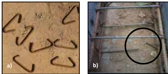
Figure 3.17 Inadequate bending of reinforcement in RC bands: a) links, and b) ties (photos: Smart Shelter Foundation)
