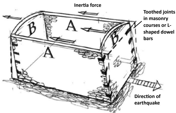
Figure 2.6 Wall connections are critical to the box-like action of a building (source: Murty 2005)
