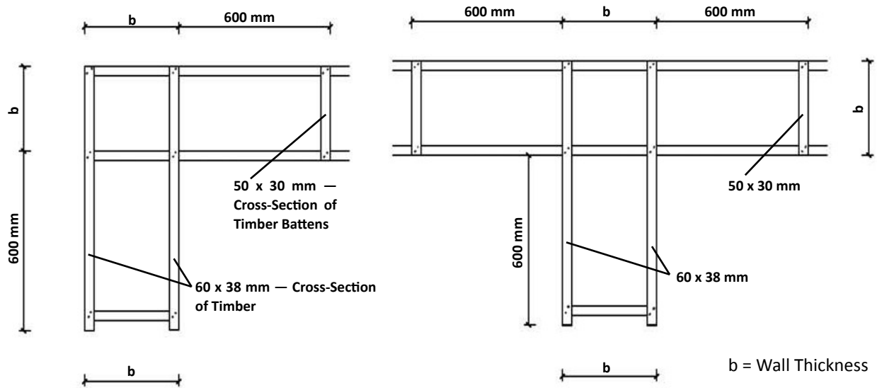
Figure 3.32 Stitches made from wood dowels at wall corners and intersections (adapted from: Bothara et al. 2002)
