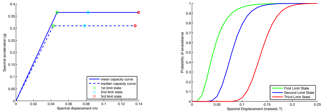
Figure 2.6 Fragility functions for Greek Frames: C4L (RC1LL)
