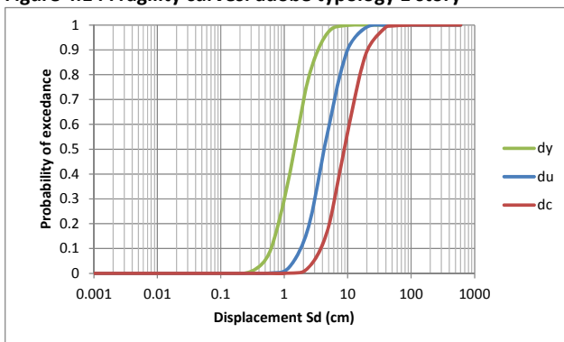
Figure 4.16 Fragility curves: rubble typology 2 story
