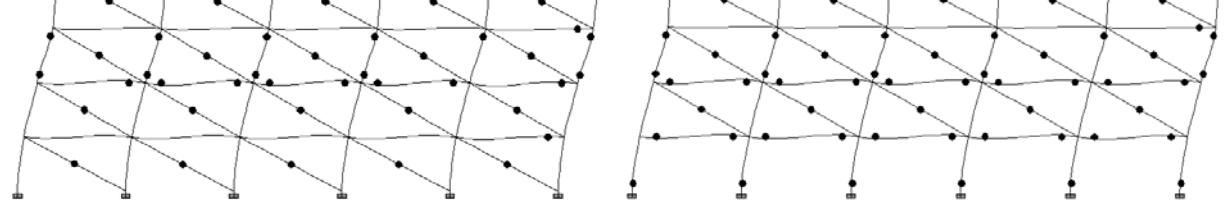
Figure 3.24 Normalized pushover curves and plastic mechanisms for bare C4M (RC_PC), infilled C3M (RC_PC) and soft story layout C3M-SS (RC_PC) Italian index frames (no seismic design, x-direction)
