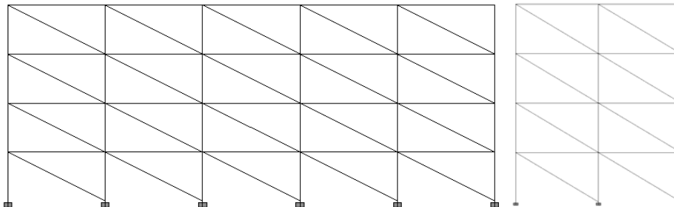
Figure 3. 23 Typical models for Italian regularly infilled index building; x-direction (left), y-direction (right)
