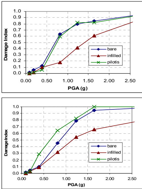
Figure 4. Evolution of economic damage (loss) index for medium-rise (top) and high-rise (bottom) buildings with R/C frame system designed to moderate codes.
