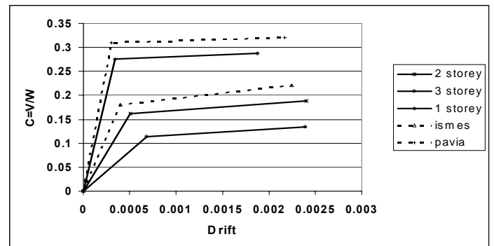
Figure 9. Pushover curves grouped per number of storeys category, and experimental curves from the literature (Pavia and Ismes tests on two-storey buildings).
