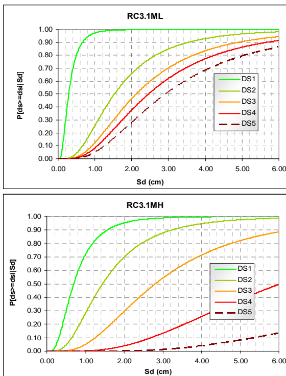
Figure 6. S_d -based fragility curves for medium-rise infilled R/C frames, low-code (top) and high-code design.
