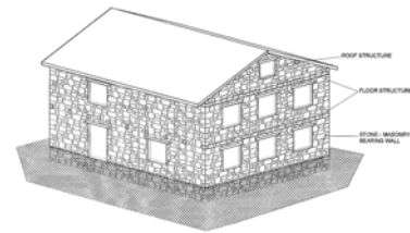
Figure 2: Key Load-Bearing Elements
