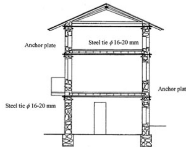
Figure 7B: Typical building elevation with seismic strengthening
