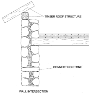
Figure 4B: Typical structural details - wall to-floor connection
