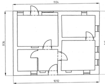
Figure 3: Plan of a Typical Building
