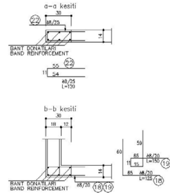
Figure 15: Strip Reinforcement for Section a-a of Figure 14
